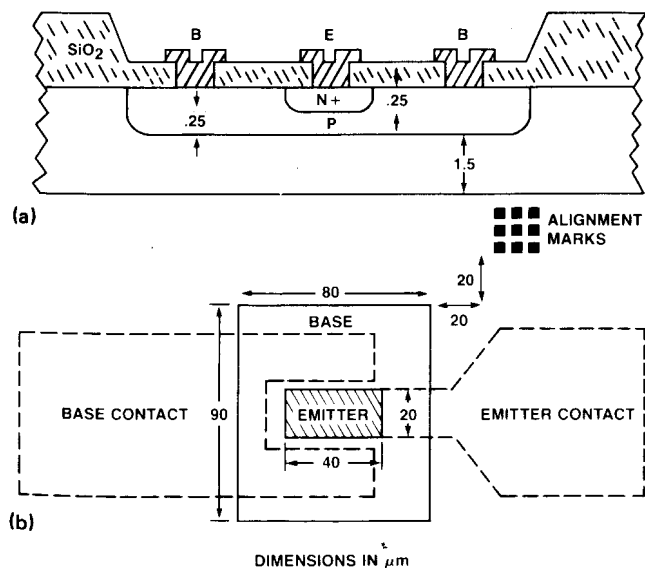
FIG. 2. Bipolar transistor structure: (a) cross-sectional view; (b) plan view.
